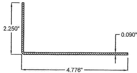
8 SILL BAFFLE
