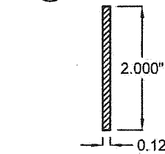
6A BLADE BRACE STRIP
