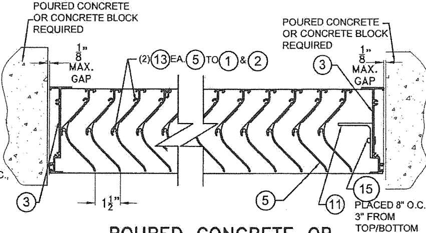
POURED CONCRETE OR CONCRETE BLOCK SUBSTRATE N.T.S.
