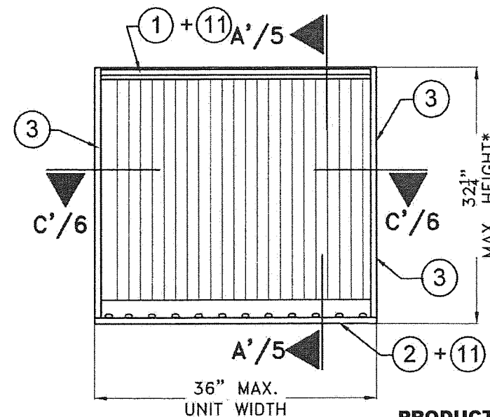
EXTERIOR ELEVATION SINGLE UNIT W/O 6A
