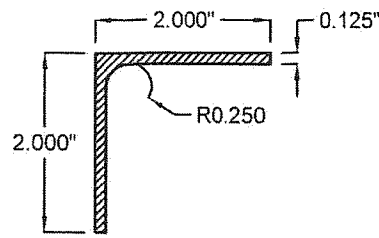
11 HEAD/SILL MOUNTING ANGLE (DOUBLES AS JAMB BLANK-OFF)
