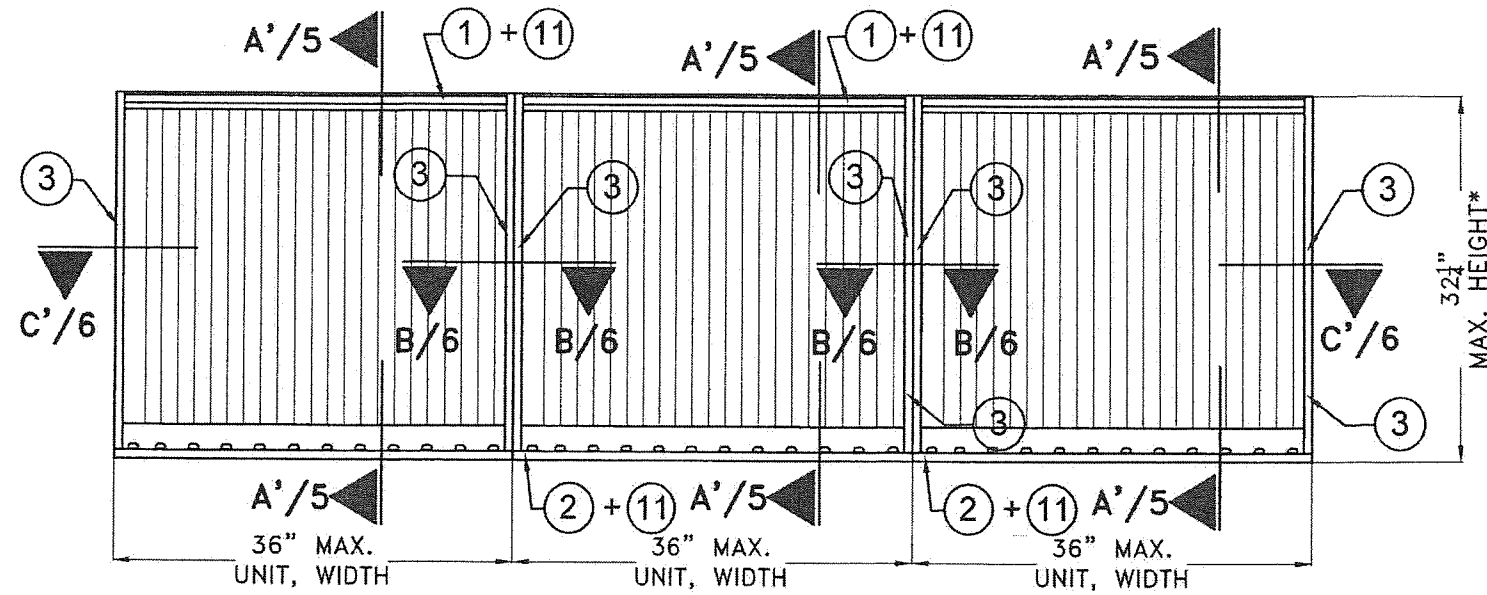
EXTERIOR ELEVATION (MULTIPLE UNITS W/O 6A)
