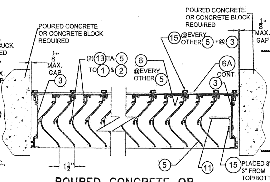
POURED CONCRETE OR CONCRETE BLOCK SUBSTRATE N.T.S.
