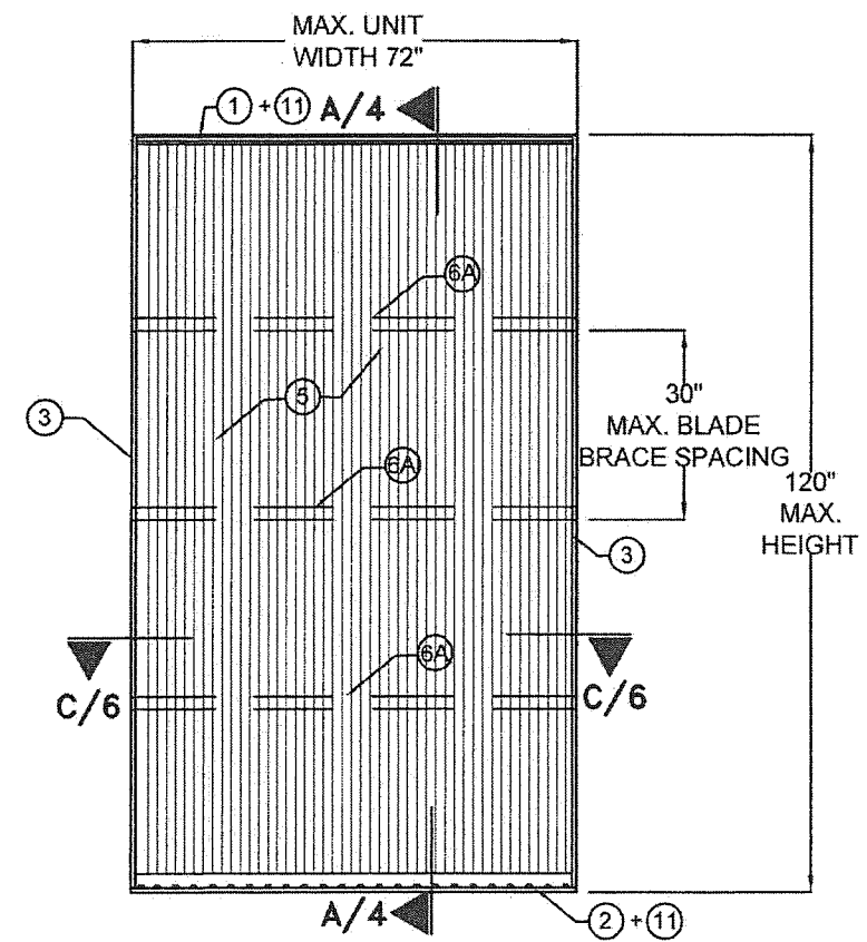
EXTERIOR ELEVATION SINGLE UNIT W/ 6A
